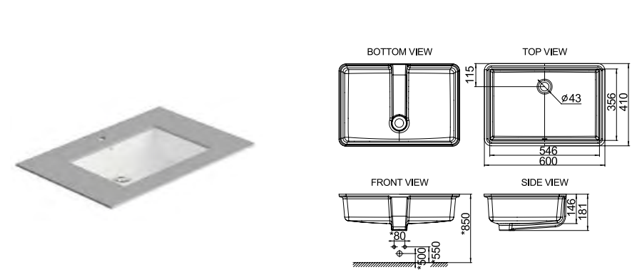
Thin Touch 下嵌型面盆 600mm CCASF513-1000410F0 L600 x W410 x H181 mm
