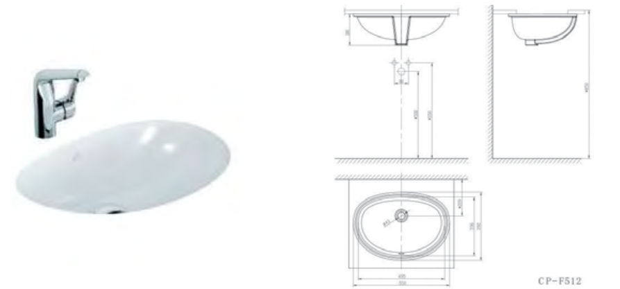
La Vita 下嵌型面盆 550mm CCASF512-1000410C0 L550 x W392 x H180 mm
