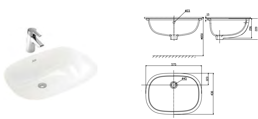
Activa 下嵌型面盆 580mm CCAS0426-1000410F0 L430 x W575 x H220 mm
