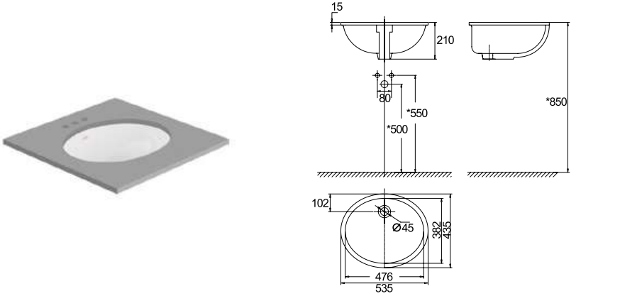
Ovalyn 下嵌型面盆 535mm CCAS0470-1000420F0 L535 x W435 x H210 mm
