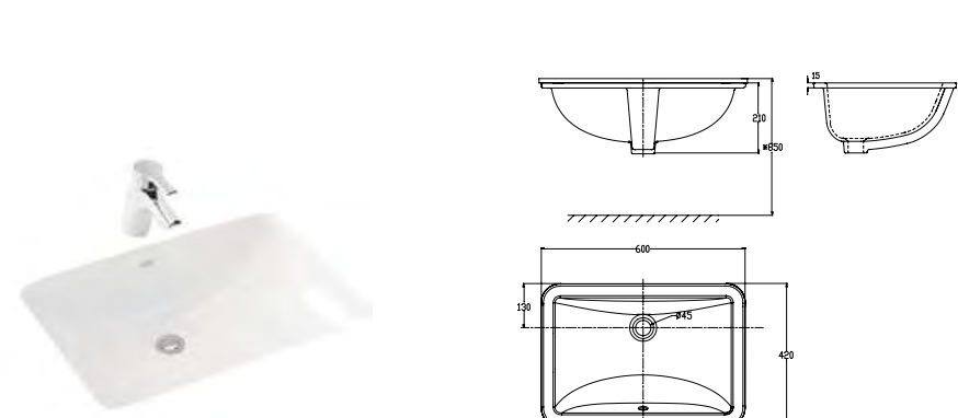
Activa 下嵌型面盆 600mm CCAS0440-1000410F0 L600 x W420 x H210 mm
