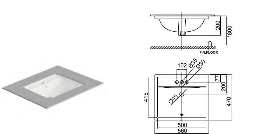
Concept 下嵌型面盆 560mm CCAS0451-1010410F0 L560 x W470 x H200 mm
