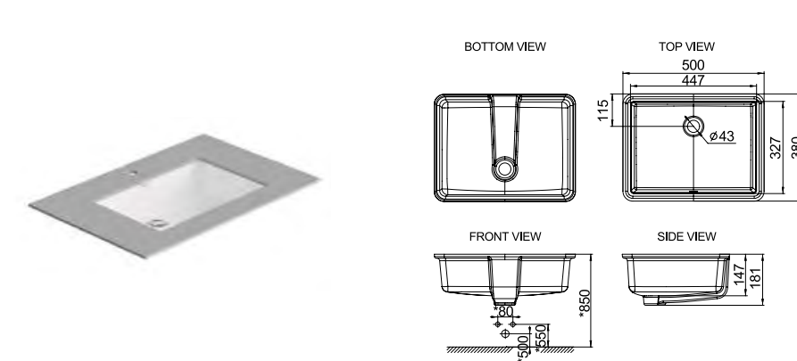
Thin Touch 下嵌型面盆 500mm CCASF514-1000410F0 L500 x W380 x H181 mm
